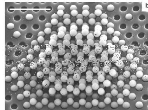
(silica spheres)
