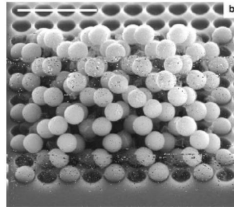
(silica spheres)
