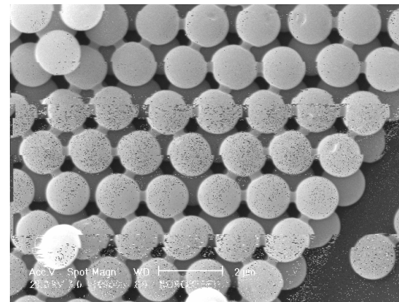
SEM images of a non-close-packing of silica colloidal crystals
