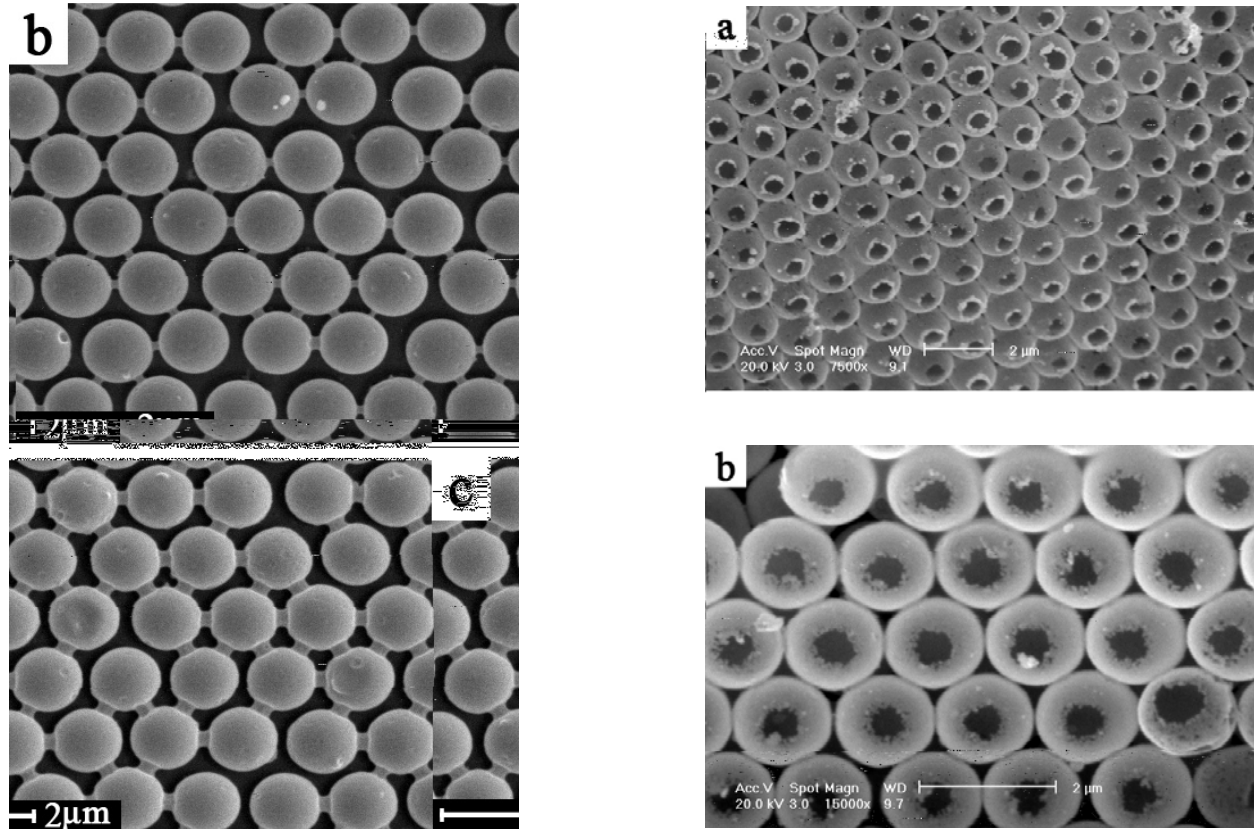
SEM images of a non-close-packing gold nanoshells
