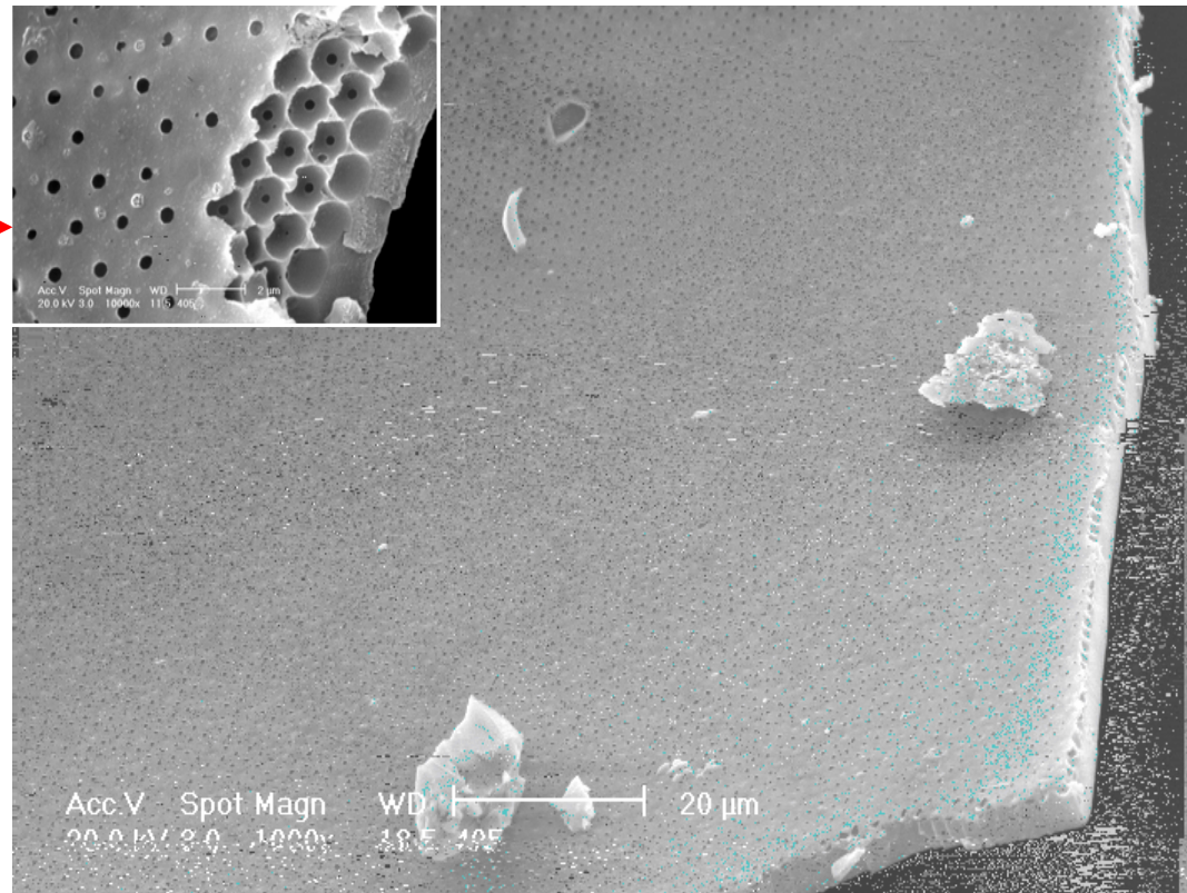
SEM images of an inverse polymer opal
